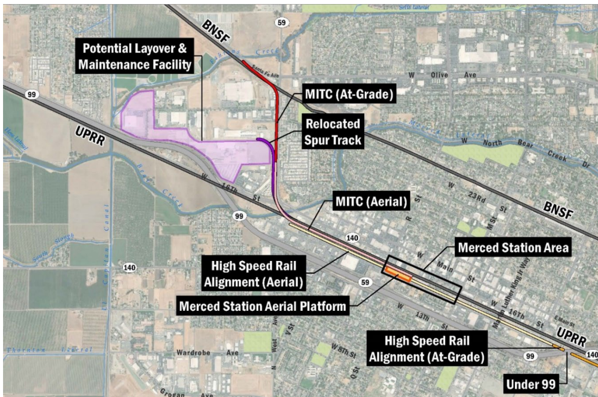
Figure 4.1 – Merced Intermodal Track Connector and Station
